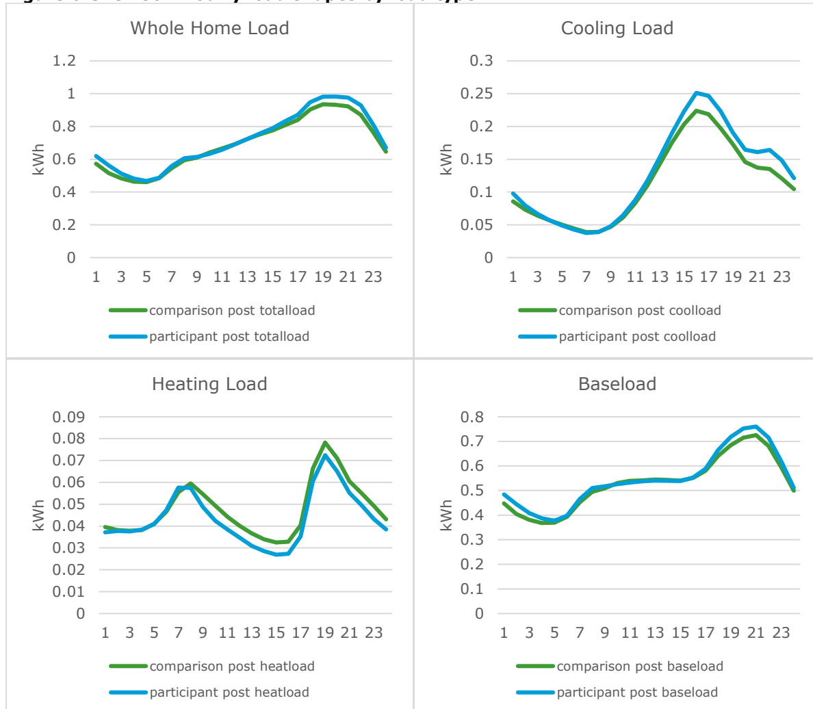
Figure 6-3. SDG&E hourly load shapes by load type
